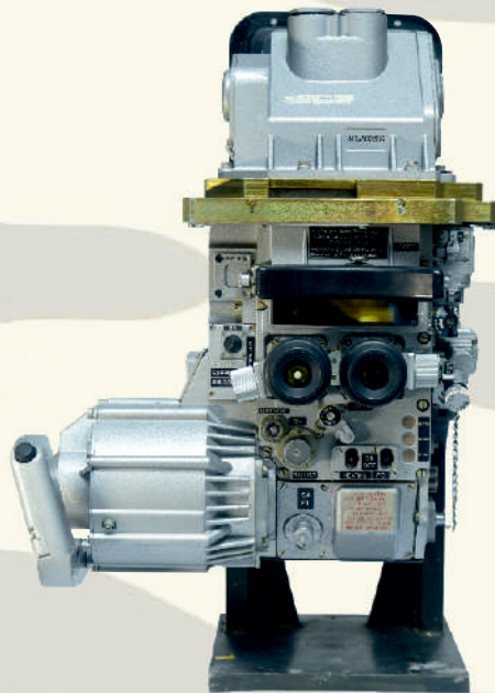
Commander Sight TKN-4S
